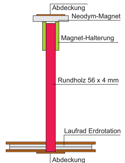
Skizze 9: Erdrotation
